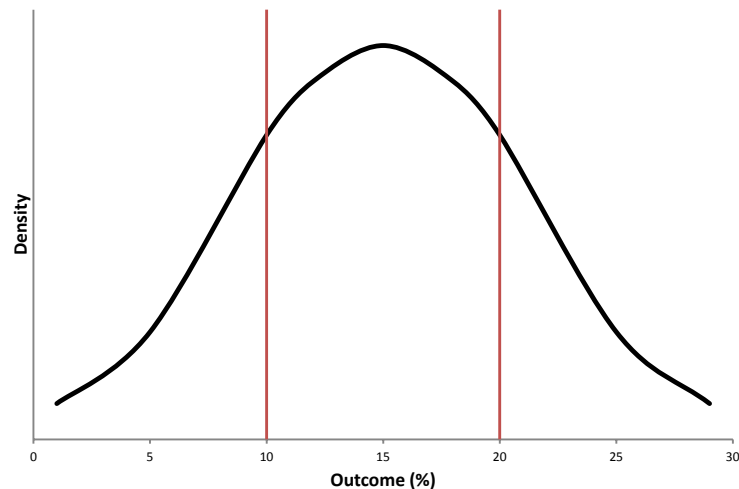
Appendix VI Figure 2. Example density plot.
